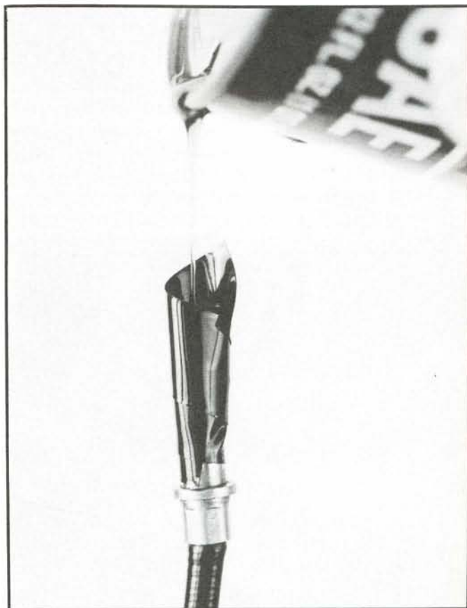
Make a funnel outta tape, pour some engine oil in it, an' have a beer while it flows into the cable.
