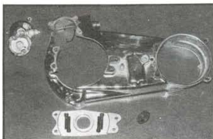
Super Max's modification service makes all the necessary changes, or you can go to your local machinist. Note that Super Max adds a third boss to the starter for more strength.
