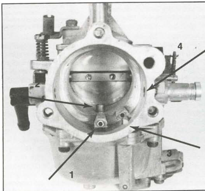
You're lookin' down the throat of a bored (40mm) and modified Keihin carb. The parts described in the text are: 1) the boss that needs to be modified (this one has been) so it won't mess up the vacuum signal to the main system spray bar; 2) the main system spray bar; 3) the tip of the accelerator-pump jet that's always pointed wrong; 4) the plugged hole where the choke shaft came through the carb (note that the mouth of the carb has been smoothed). This thing passes a lotta gas.
