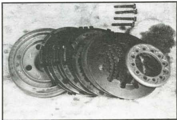
Harley's Evolution clutch is sure different from the traditional one. It'll handle more torque, but not more heat. The left photo shows all the parts of the new clutch. Center is a shot of the assembly; notice the automotive-style diaphragm spring. The aluminum collar that compresses the spring (right photo) also adjusts the spring shape, which is critical for best clutch feel and performance.
