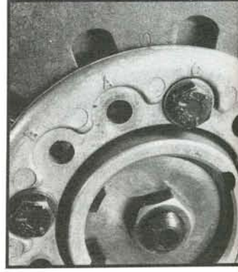
Harley's Evolution clutch is sure different from the traditional one. It'll handle more torque, but not more heat. The left photo shows all the parts of the new clutch. Center is a shot of the assembly; notice the automotive-style diaphragm spring. The aluminum collar that compresses the spring (right photo) also adjusts the spring shape, which is critical for best clutch feel and performance.
